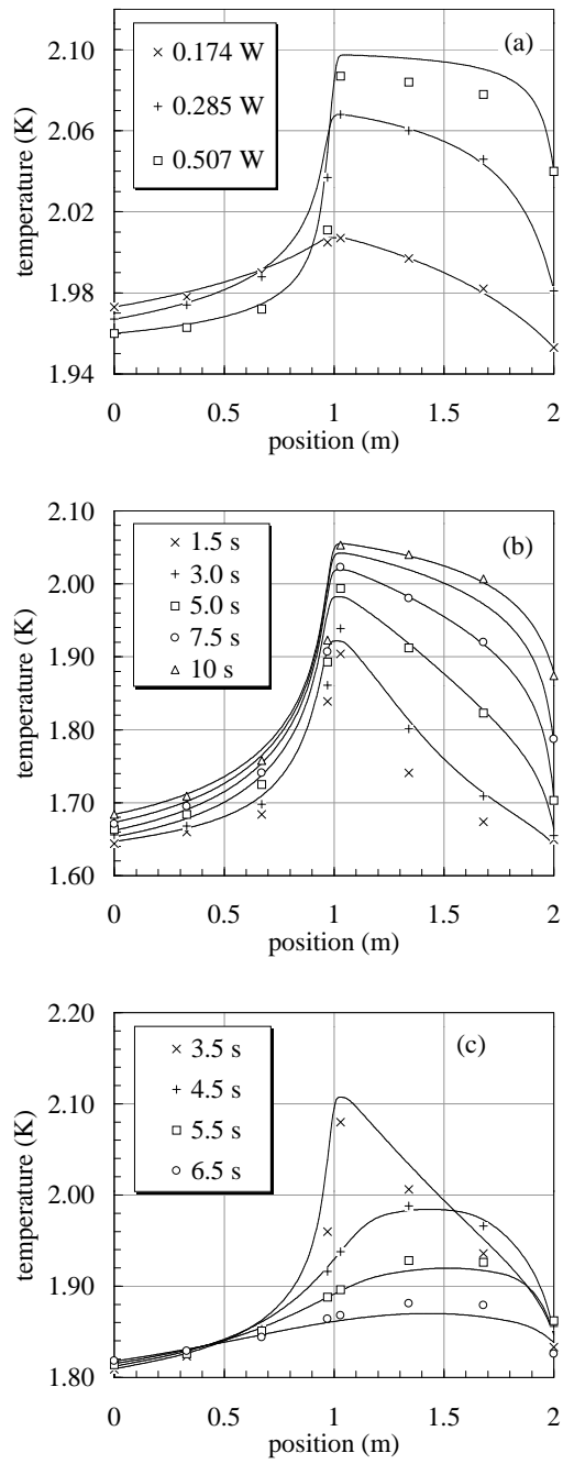
Figures 4. Comparison of experimental steady-state (a) and transient heat input ((b) and (c)) data from Kashani et al.[12] to the results of simulations.
