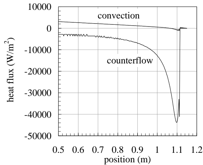
Figure 7. Heat fluxes due to the counterflow heat exchange mechanism in superfluid helium and due to convection, as computed at t=0.1 s in the simulation of the experiment of Lottin and Van Sciver [18].
