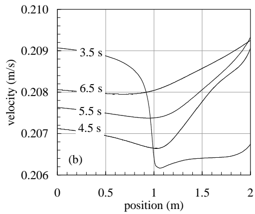
Figures 5. Calculated velocity at different times (indicated on the curves) for the transient heat input simulations of the experiments of Kashani et al.[12], (a) refers to a step in heating power, (b) to a rectangular heating pulse.
