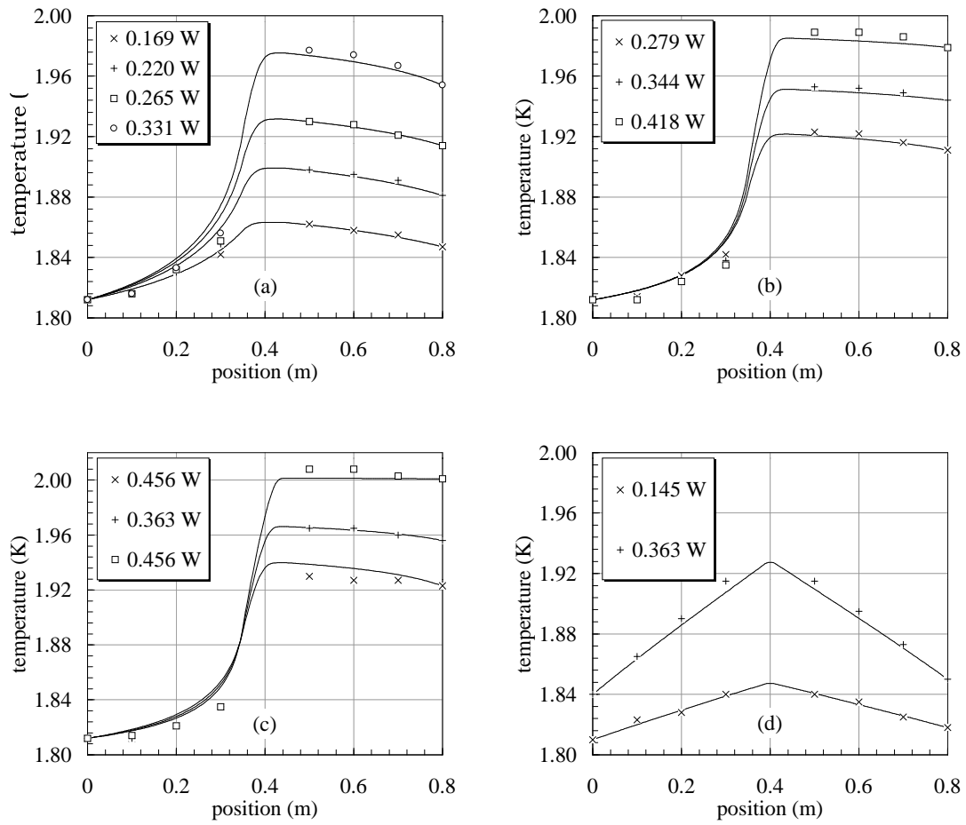
Figure 3. Comparison of experimental data from Srinivasan and Hoffman[17] with simulations. The results are grouped by operating pressure and massflow: (a) 2.5 bar and 0.329 g/s, (b) 5 bar and 0.347 g/s, (c) 7 bar and 0.334 g/s (d) 1 bar stagnant. Heater powers as indicated in the legends.
