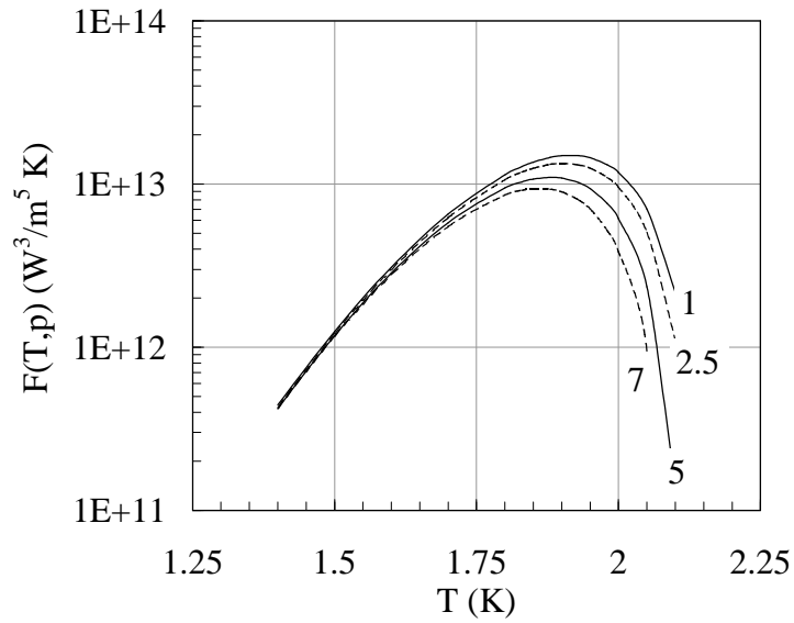
Figure 1. Superfluid heat conductivity function F(T,p) at several pressures (indicated in bar on the curves). The function F(T,p) is zero above the lambda temperature T_\lambda (in the range of 2.1 K)
